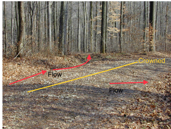
Crowning and cutouts promote good drainage and stable permanent access roads.
