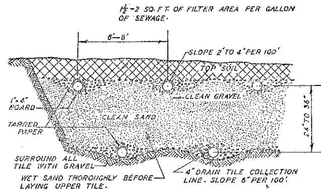
SECTION OF ARTIFICIAL ABSORPTION BED
