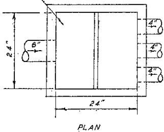
DETAILS OF DIVERSION BOX
