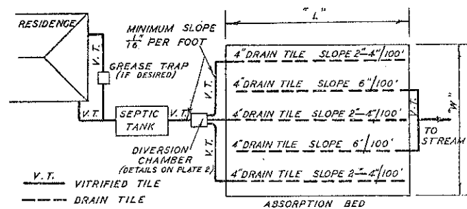
TYPICAL LAYOUT FOR SINGLE RESIDENCE
