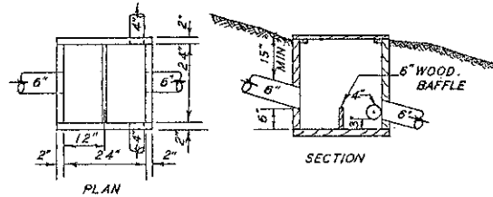
DETAILS OF DIVERSION BOX
