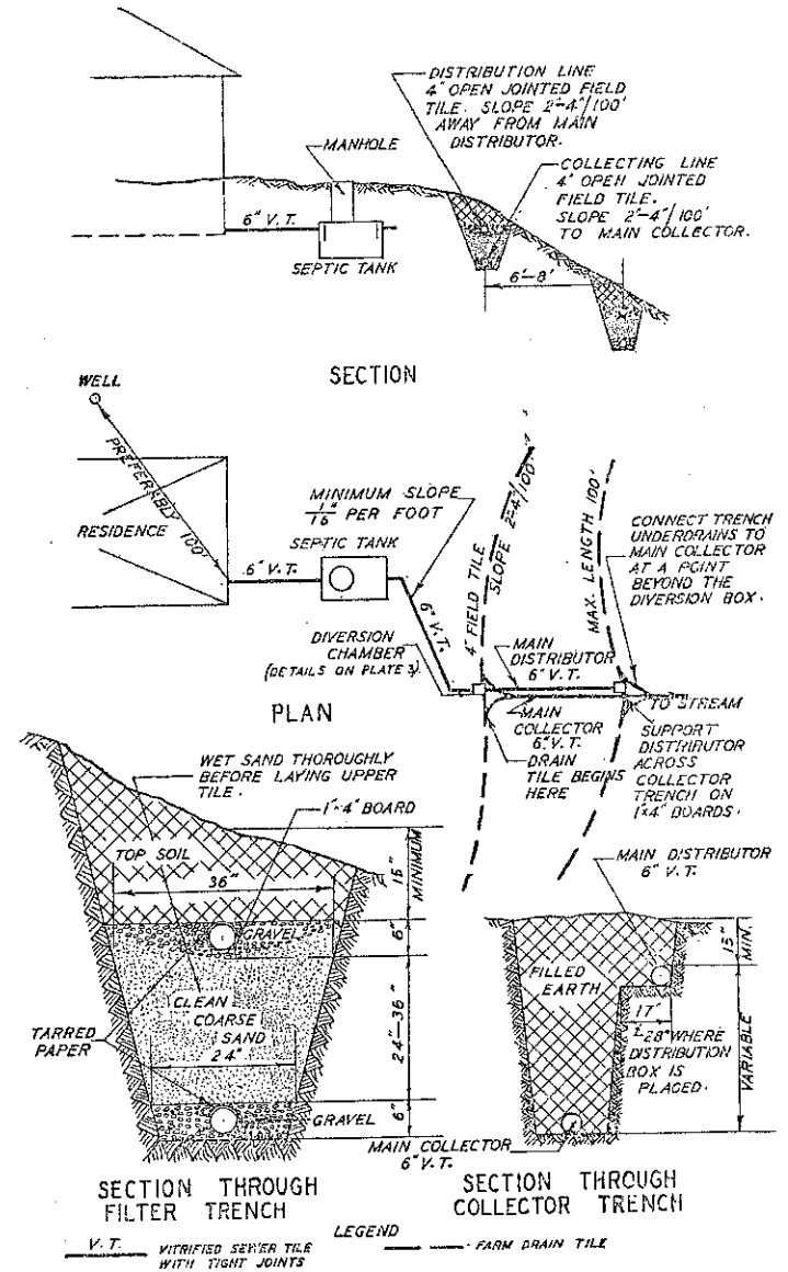
Trench Filter Plate No. 5
