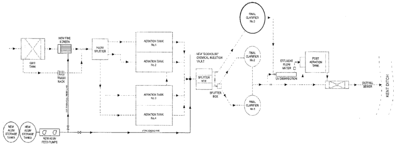
PROCESS FLOW SCHEMATIC
