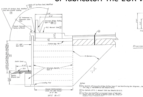
Figure 10-1 Example MSE Wall Plans
