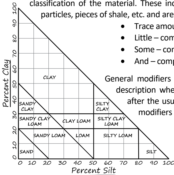
Figure 2-1 Soil Classifications
