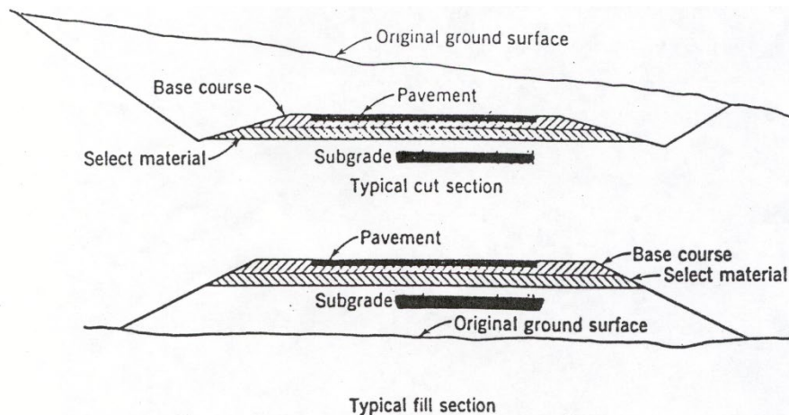
Figure 7-1 Typical Roadway Cross Sections
