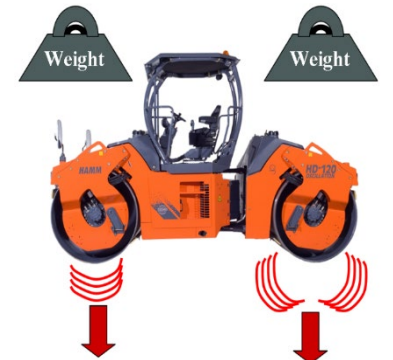
Figure 3-13 Oscillatory Roller
