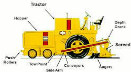
Figure 3-3 Paver Components
