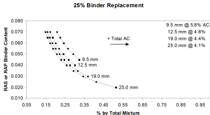
Figure 2-3 Binder Replacement
