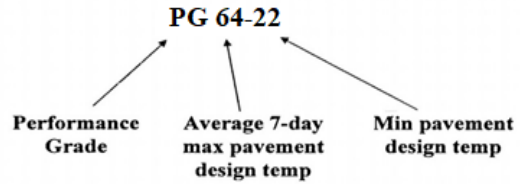
Figure 1-3 PG Grading System
